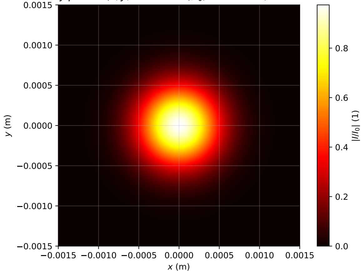
Intensity profile I(x, y, z = 0.398m)/I_0 , P_{in}=0.1P_{cr} , artificial time
